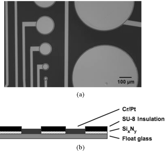
Fig. 1. (a) Photolithographically fabricated Pt MEA with varying disk radius. (b) Corresponding cross-sectional schematic.
